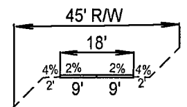
TYPICAL STREET SECTION - NTS - HOLLYDALE
