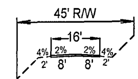
TYPICAL STREET SECTION - NTS - CEDARDALE & FERNDALE
